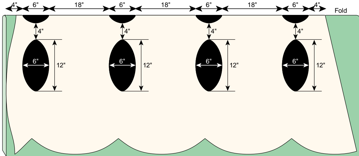
CATERPILLAR DIAGRAM
